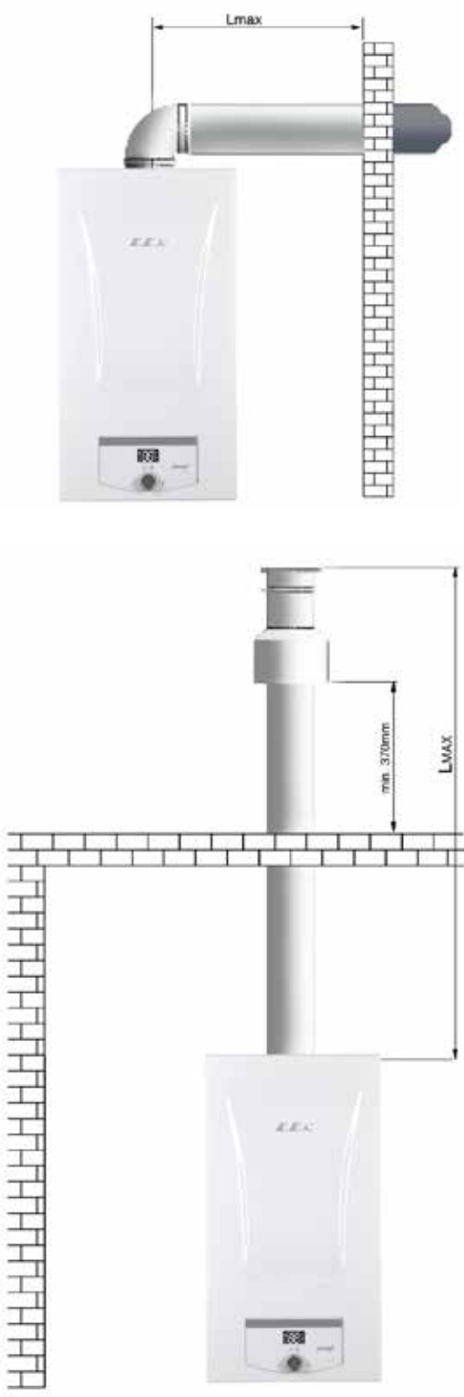
Horizontal Hermetic Flue Application L max. distance with single elbow: 4 m, 60/100
